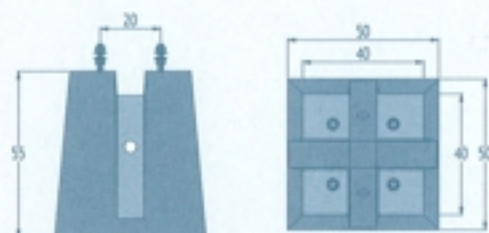
Massif 50 x 50
