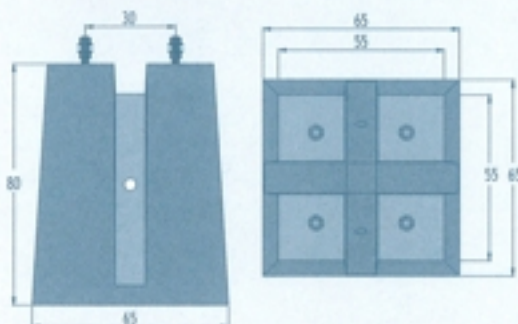
Massif 65 x 65
